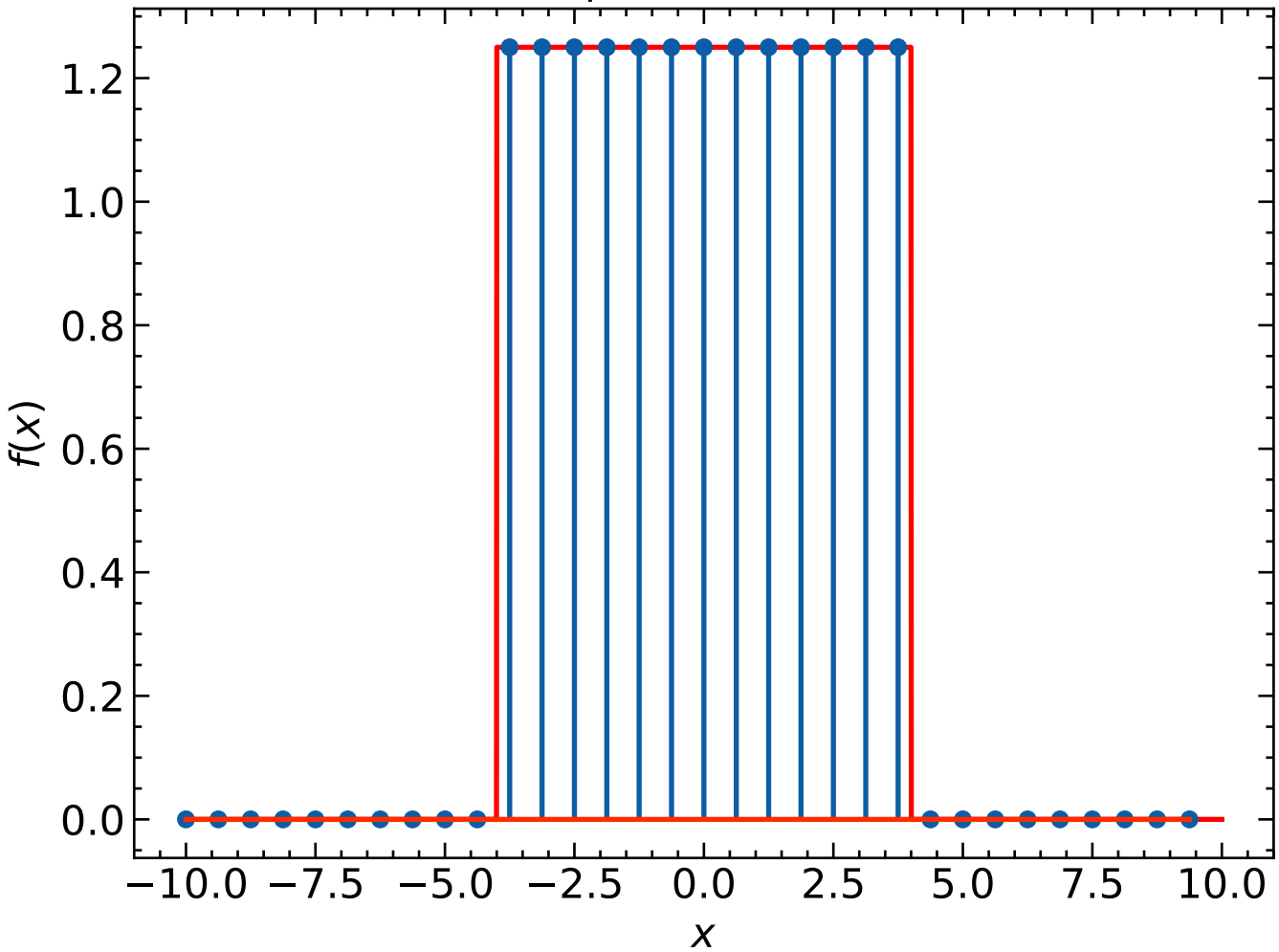
Space domain
