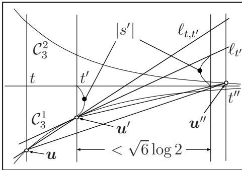
Figure 3: Triangle across Axis.
