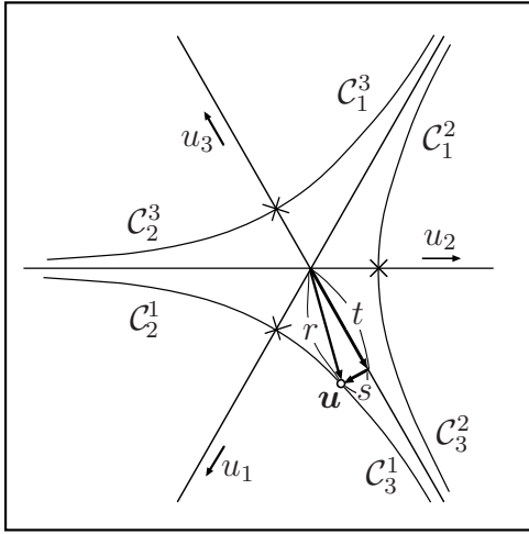
Figure 1: The Continuous Curve \mathcal{C} .
