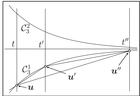
Figure 4: Triangle in One Side.
